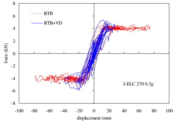
Figure 10 Force-displacement loops.
