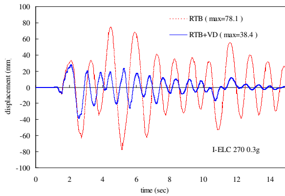
Figure 9(b) Displacement time histories.
