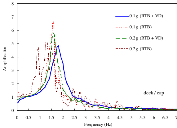
Figure 7 The deck-to-cap beam transfer function.
