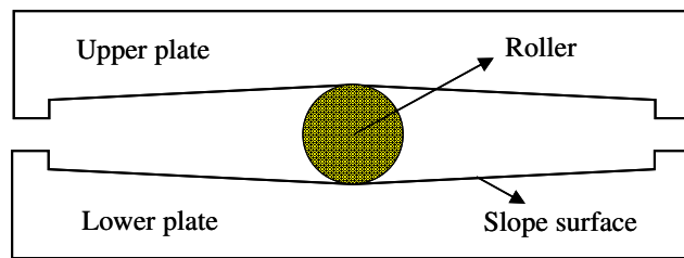
Figure 1 A schematic of the RTB unit.
