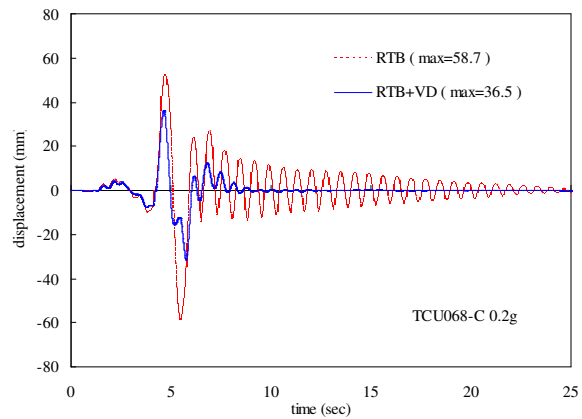
Figure 11(b) Displacement time histories.
