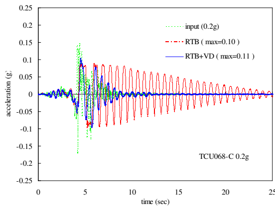
Figure 11(a) Acceleration time histories.
