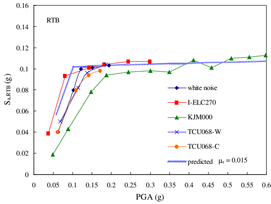
Figure 12 Peak deck acceleration (RTB).
