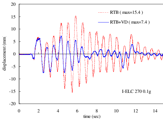
Figure 8(b) Displacement time histories.
