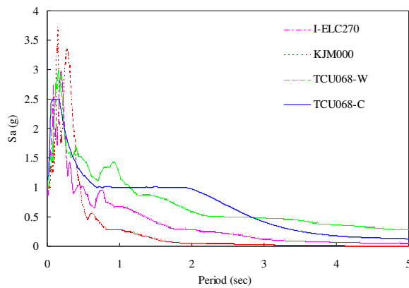
Figure 5 Normalized input response spectra.
