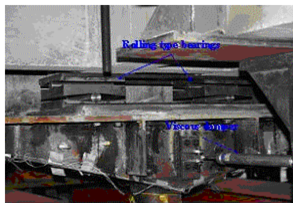
Figure 4 The RTB assembly and viscous damper.
