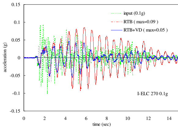
Figure 8(a) Acceleration time histories.
