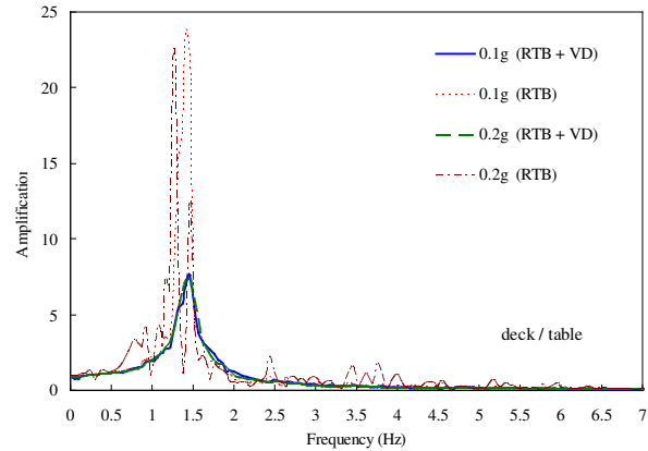
Figure 6 The deck-to-table transfer functions.
