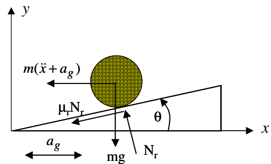
Figure 2 External forces acting on the roller.
