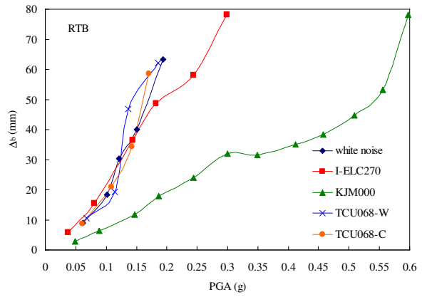
Figure 13 Peak bearing displacement (RTB).
