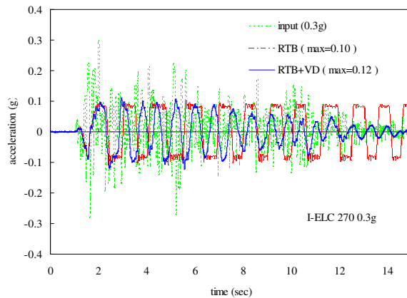
Figure 9(a) Acceleration time histories.
